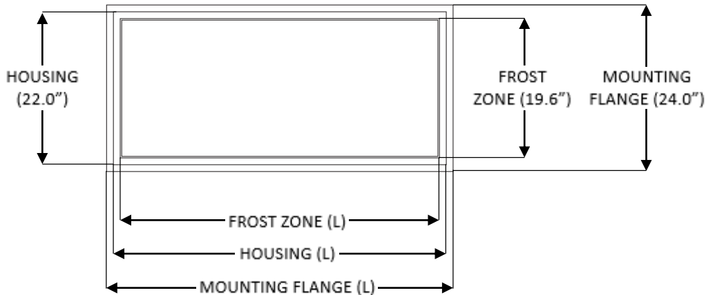
FRONT VIEW
