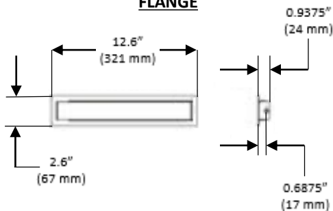
INTAKE COUNTER FLANGE
